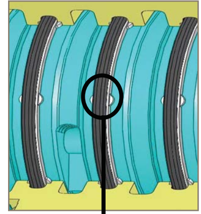
Locking tab
